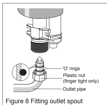
Figure 8 Fitting outlet spout
