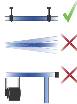
Fig. 11 Fixing the pipes
