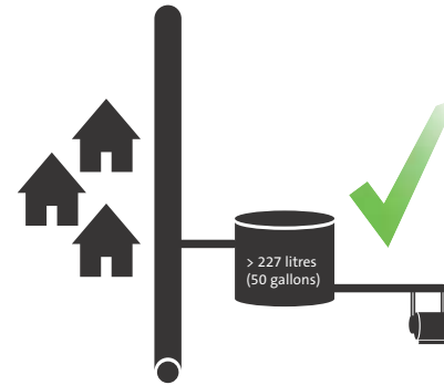
Fig. 2 Connection to mains via storage tank
