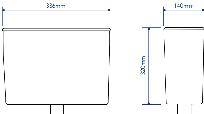
Shown: Concealed pneumatic cistern with brushed stainless steel push plate BTWPNEUMBSS
